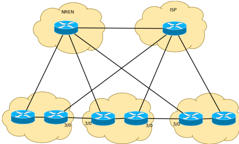
Figure 2: Peering Topology
