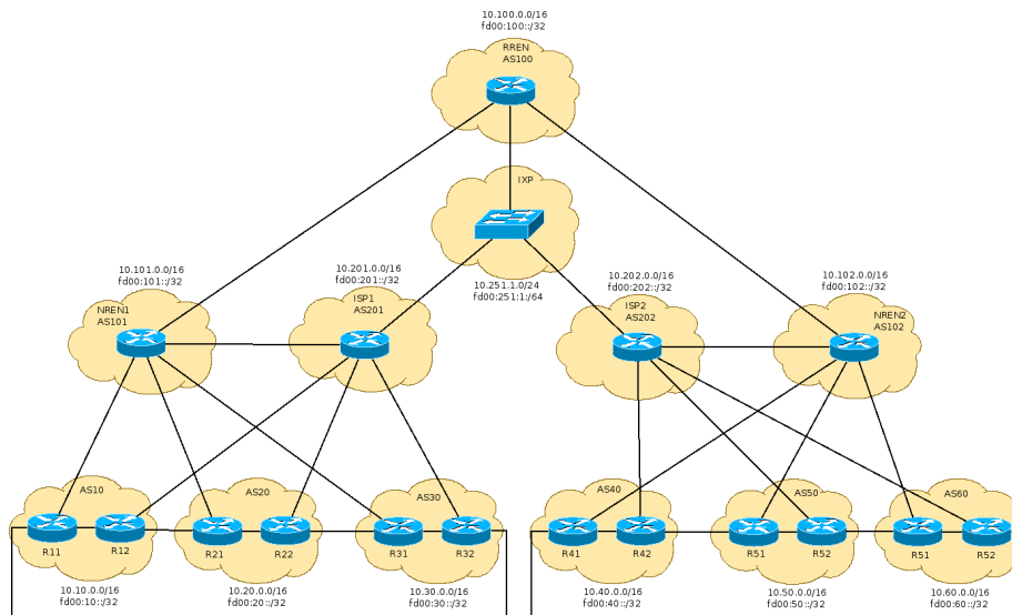
Figure 1: Multi-homed Topology
