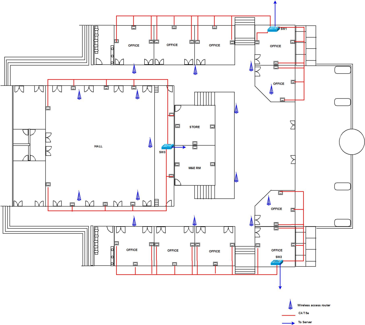
GROUND FLOOR PLAN-A WITH PHYSICAL DIAGRAM
