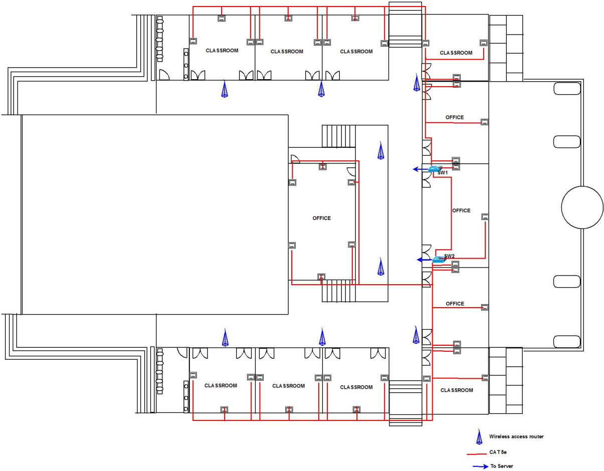
SECOND FLOOR PLAN WITH PHYSICAL DIAGRAM
