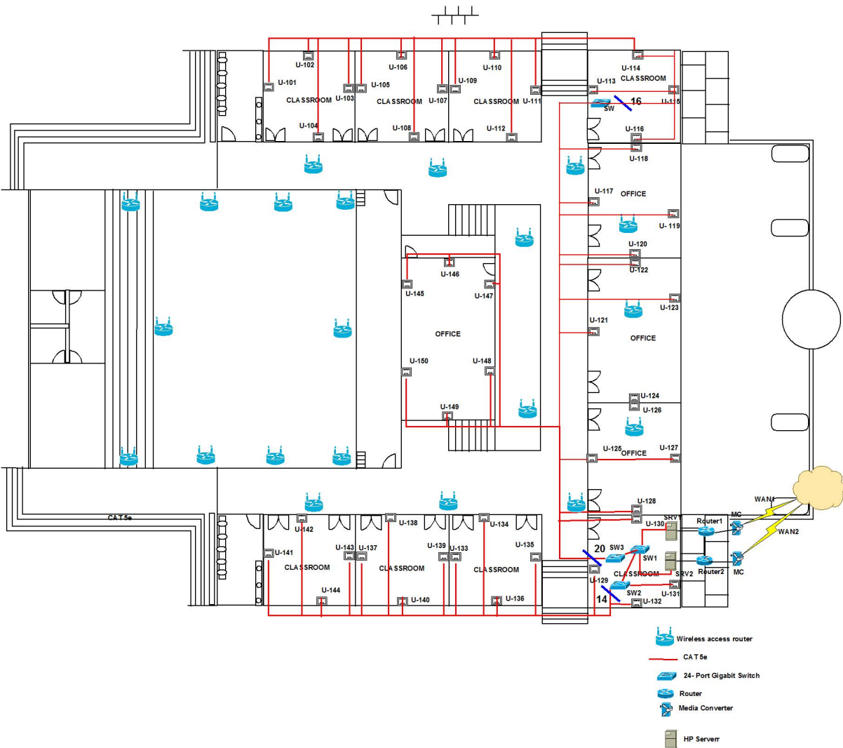
FIRST FLOOR PLAN WITH PHYSICAL DIAGRAM
