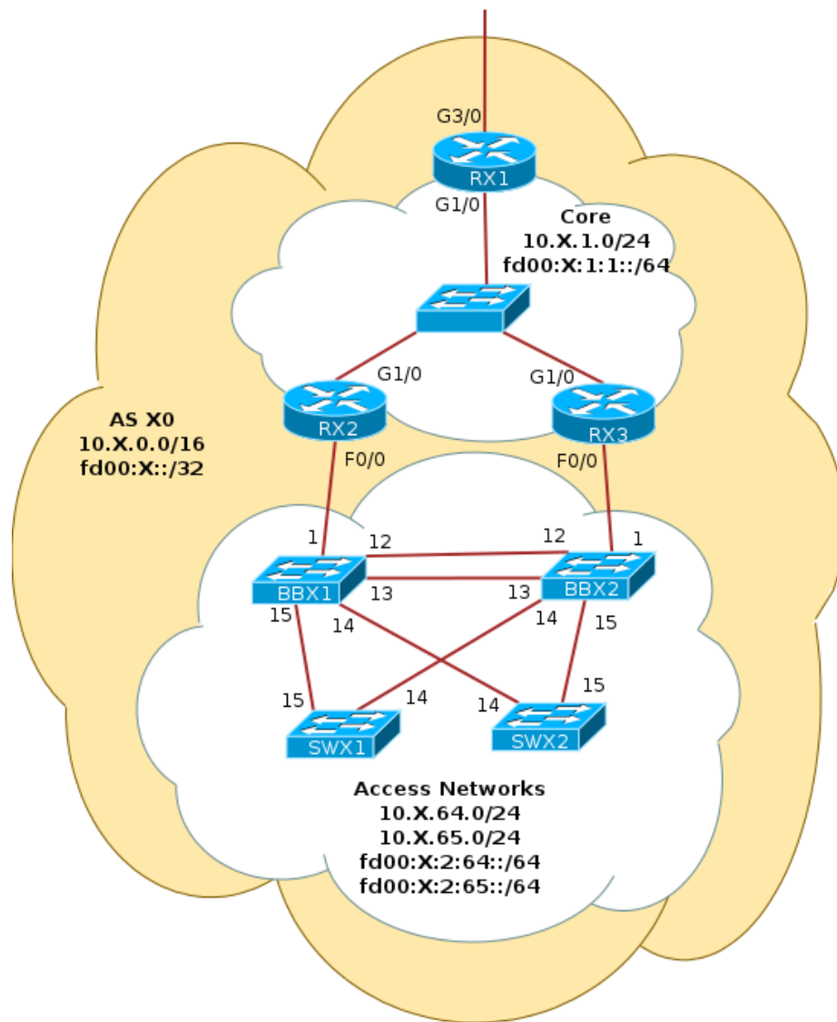
Figure 1: Physical Topology
