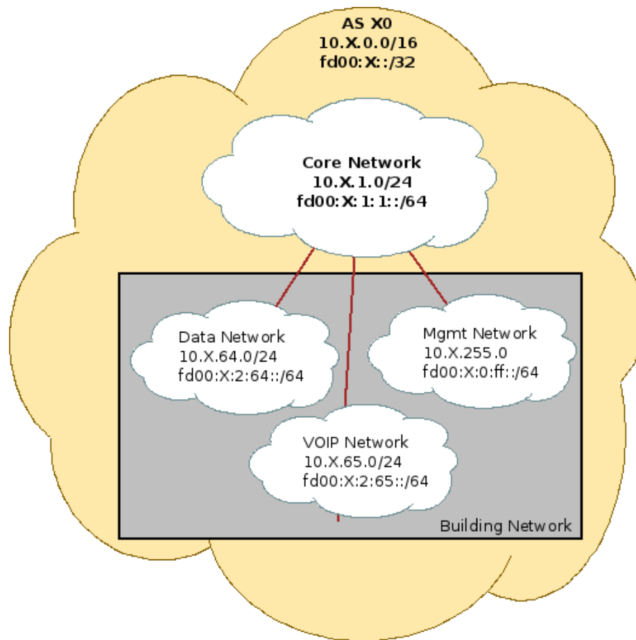
Figure 1: Logical Topology
