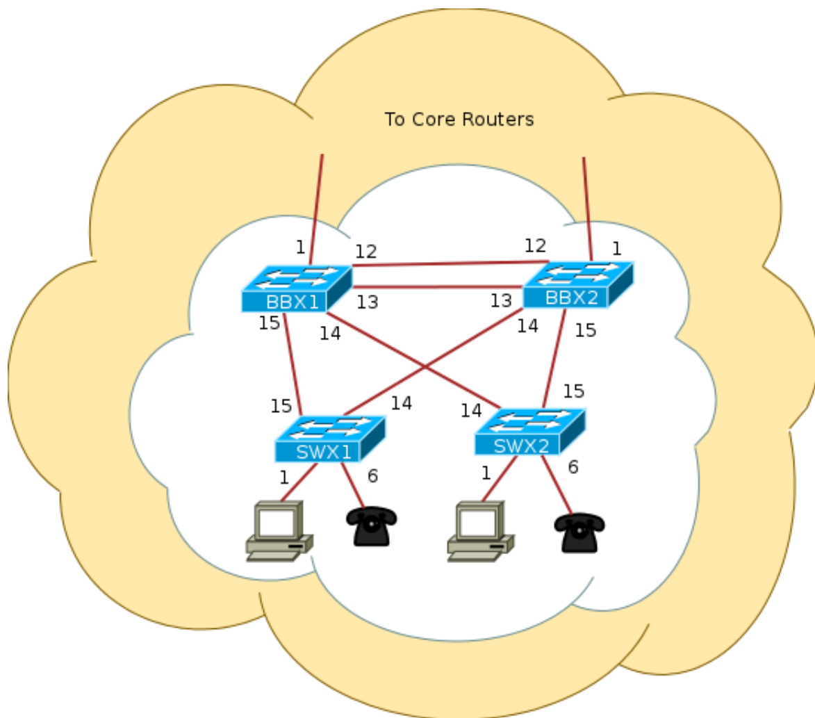
Lab topology
